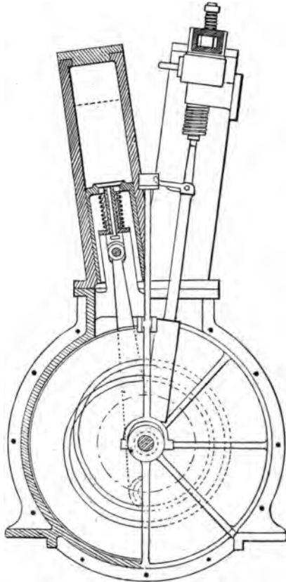
FIG. 202.—Part sectional view of the Daimler V-shaped Gasoline Engine, showing the air valve in the piston for admitting air at the suction stroke, and eccentric cam grooves on the fly-wheel disc. The method of opening the exhaust valve is also indicated. The push rod of the exhaust valve carries a feather at its lower end, which travels on the eccentric cam grooves indicated on the face of the piston. Under impulse from the centrifugal governor, at high speed, the feather follows an approximately circular path, thus preventing the push rod from lifting and pushing the valve rod, to open the valve.
